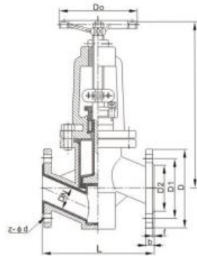
Fluorine lining valve ( J41F46 )
