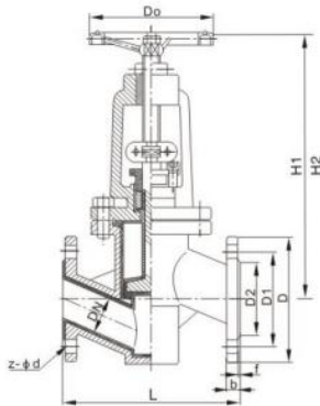
Fluorine lining valve ( J41F46 )
