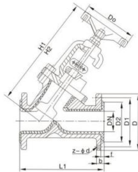
Fluorine lining valve ( J45F46 )
