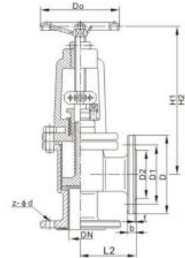
Fluorine lining valve ( J44F46 )
