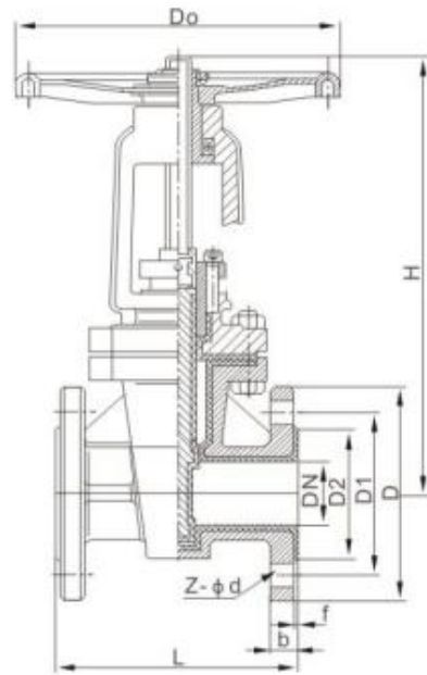
Fluorine valve(Z41F46)
